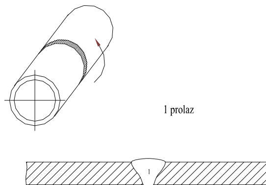
Raspored zavara
